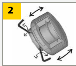
Adjust the tilt angle of the detection field with the hex key.
